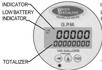
TYPICAL FORWARD DIGITAL INDICATOR-TOTALIZER
