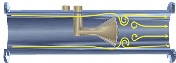
Figure 2: The V-Cone's Vortices
