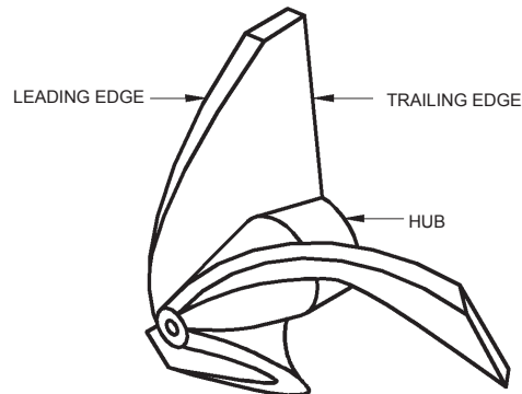
Figure: 16 Propeller Elements
