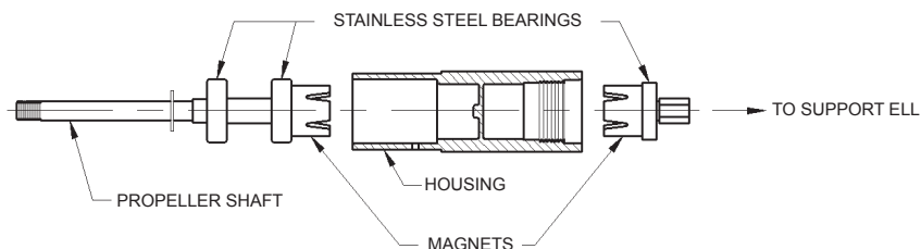
Figure: 12 Bearing Assembly
