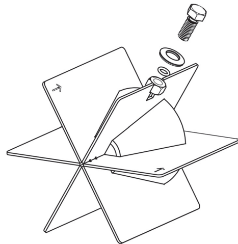
Figure: 8 FS100 Flow Straightener
