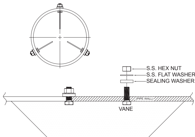
Figure: 7 Bolt In Straightening Vanes
