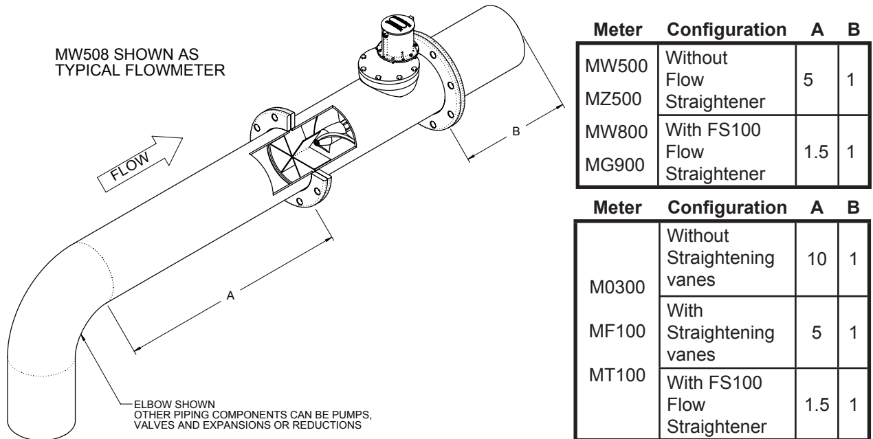
Figure: 5 Installation Requirements
