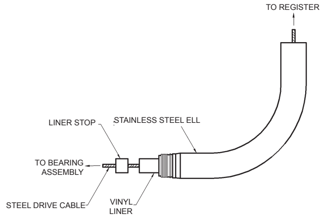
Figure: 13 Drive Assembly
