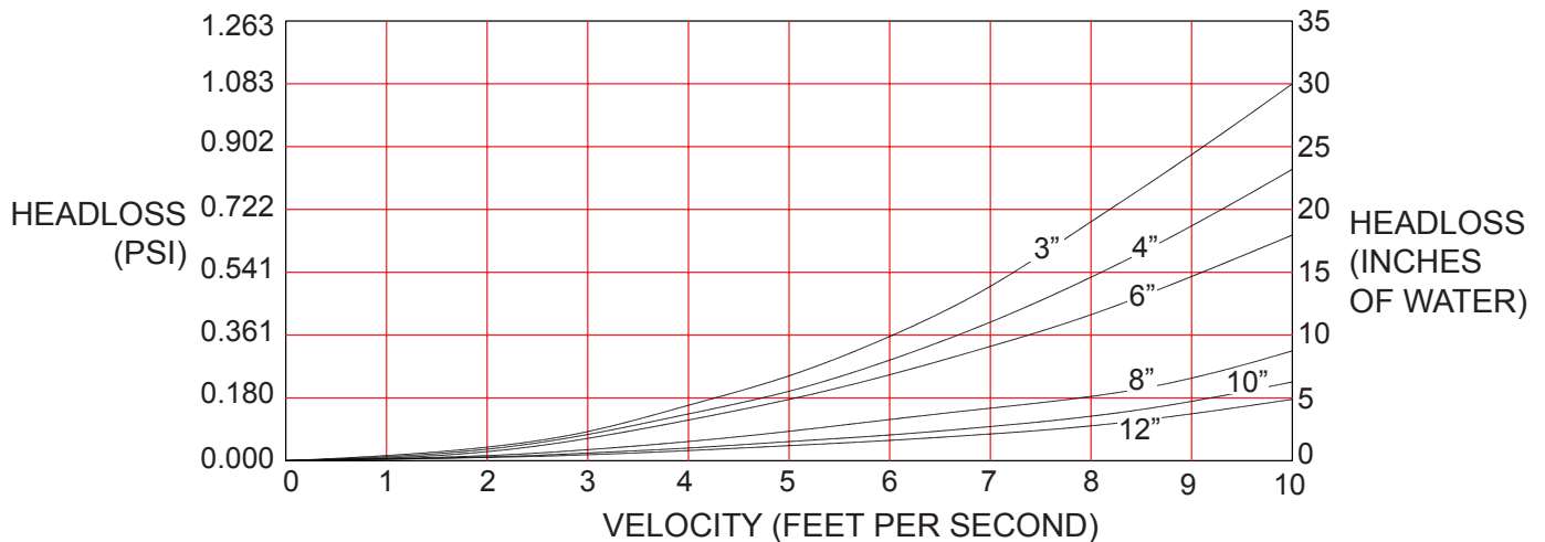
HEADLOSS CHART
