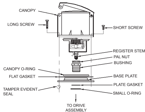
Figure: 14 Meterhead
