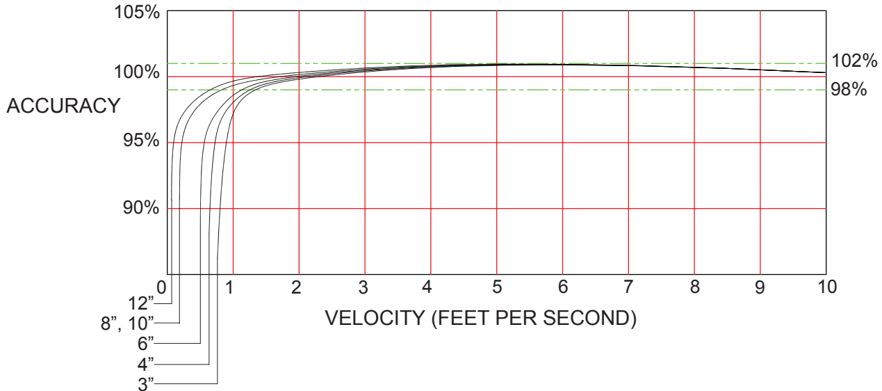
ACCURACY CHART
