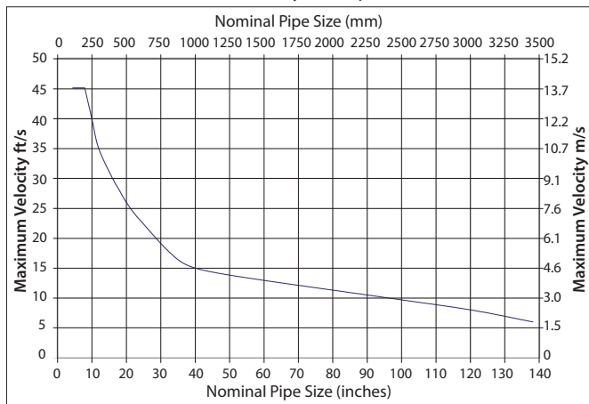
Maximum Velocity For Pipe Sizes
